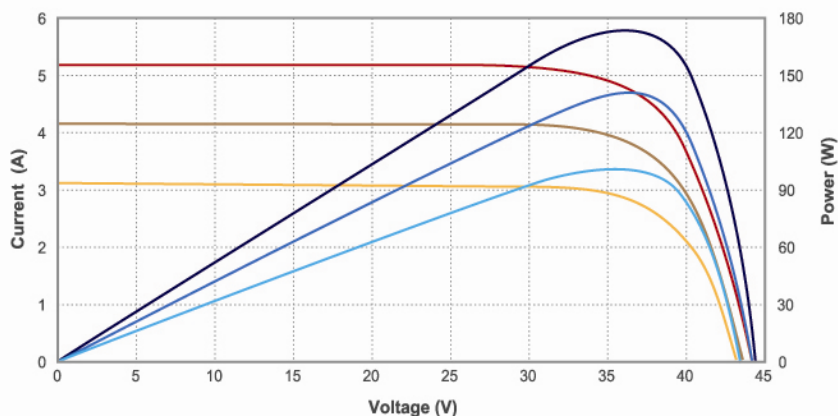
Current Power v.s. Voltage Characteristics
